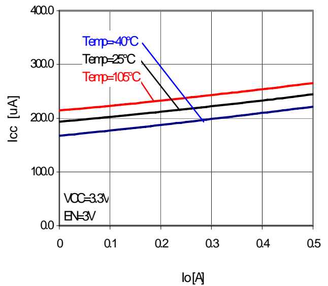
Figure 30. I_O-I_{CC}
