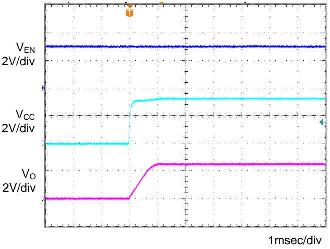
Figure 10. Input sequence 1 Co=1µF,Ta=25°C
