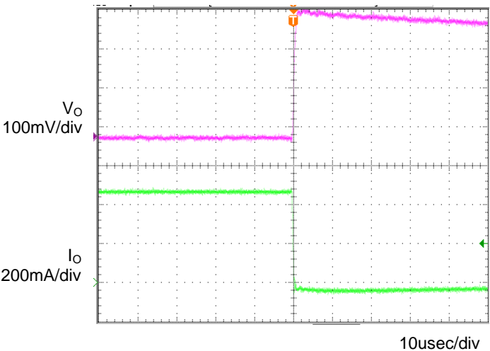
Figure 8. Transient Response (0.5→0A) Co=1µF,Ta=105°C
