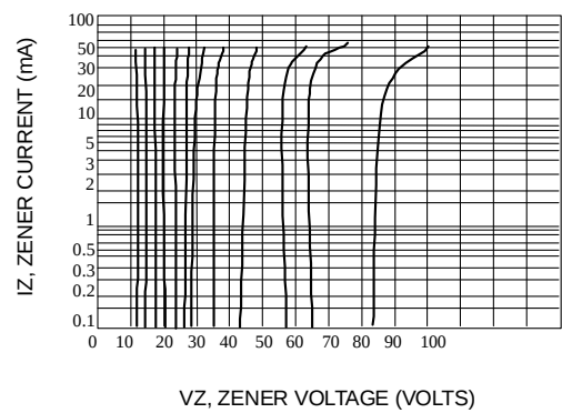
Fig. 8-VZ = 12 THRU 82 VOLTS
