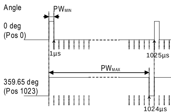
Figure 6: PWM duty cycle depending on magnet position
