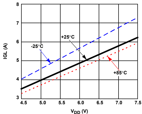
FIGURE 13. LS PULL-DOWN CURRENT WITH TEMPERATURE ( V_{GL} = 2.5V , LSEL = VDD)
