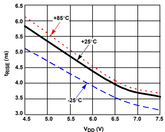
FIGURE 15. t_{RL} WITH TEMPERATURE ( C_{GL} = 3nF , LSEL = VDD)
