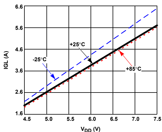
FIGURE 11. LS PULL-UP CURRENT WITH TEMPERATURE ( V_{GL} = 2.5V , LSEL = VDD)
