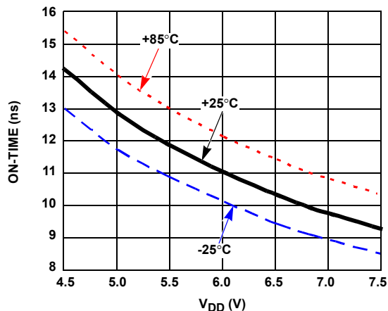
FIGURE 7. t_{GH,ON} WITH TEMPERATURE (CGH = 0) (see Figure 3 for t_{GH,ON} timing)
