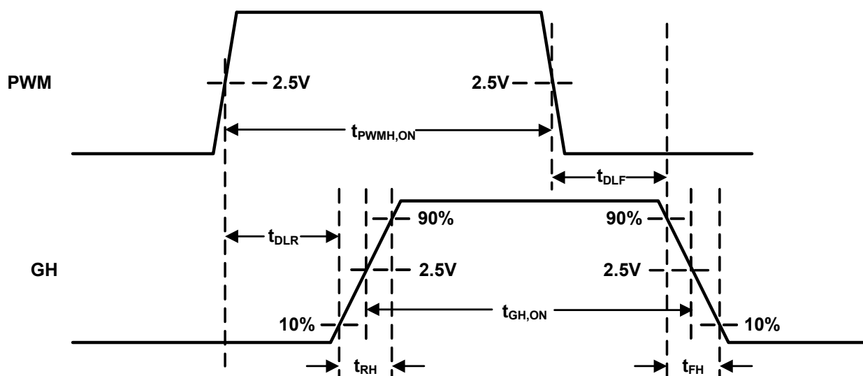
FIGURE 3. TIMING DIAGRAM
