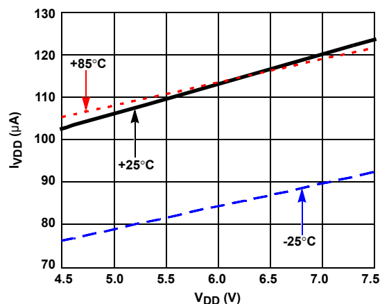
FIGURE 4. I_{VDD} vs V_{DD} WITH TEMPERATURE (NO SWITCHING)
