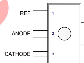
PK PACKAGE (Top View)
