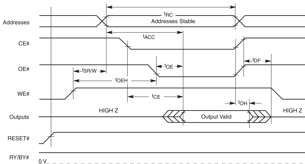
Figure 15.1 Read Operations Timings
