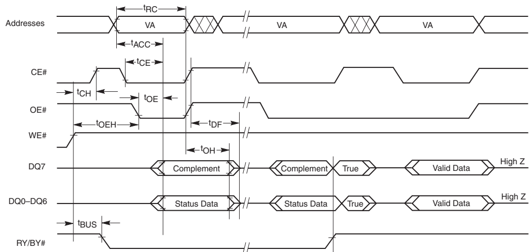
Figure 15.8 Data# Polling Timings (During Embedded Algorithms)
