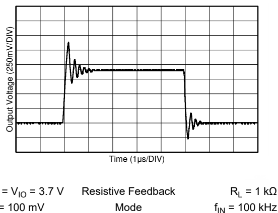
Figure 6-6. LNA Response
