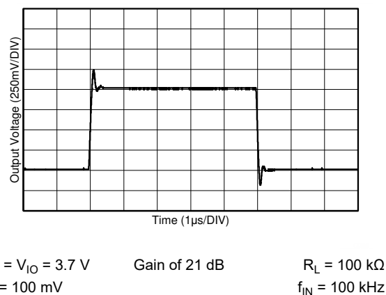
Figure 6-7. PGA Response
