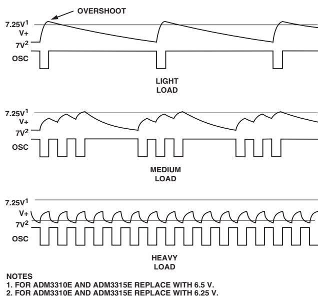
Figure 4. Operation of Green Idle Under Various Load Conditions
