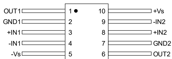
Figure 2. Pin Assignments - Top View
