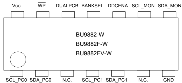
Fig.16 Pin Layout
