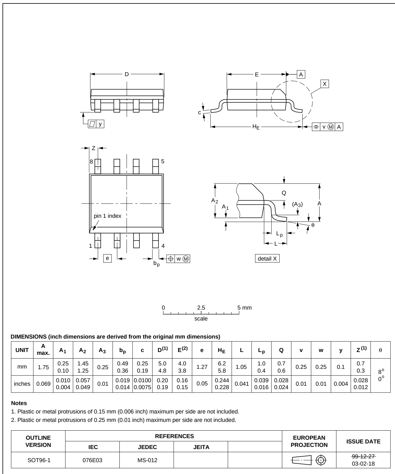
Fig 7. Package outline SOT96-1 (SOT8)
