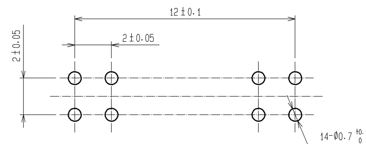
RECOMMENDED PC BOARD HOLE PATTERN
