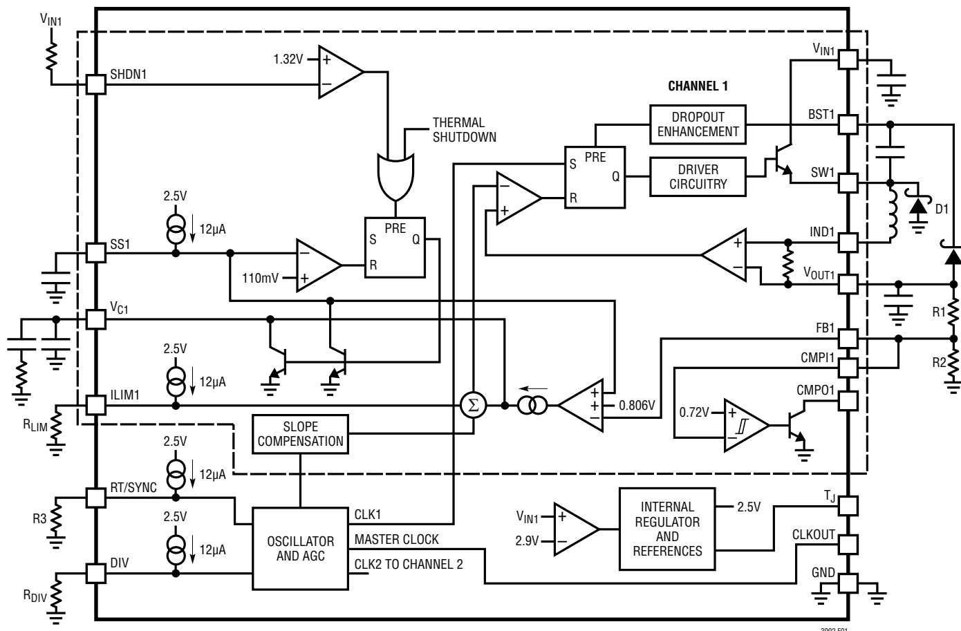
Figure 1. LT3992 Block Diagram
