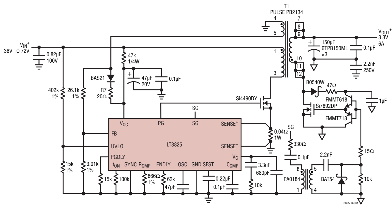
48V to 3.3V at 6A Isolated Supply
