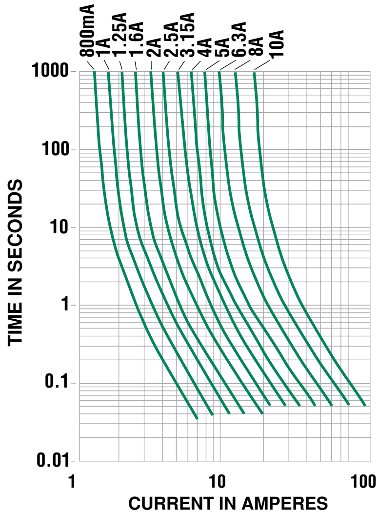
Average Time Current Curves
