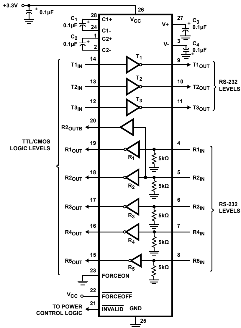
FIGURE 3. ICL3245E
