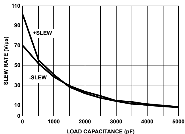
FIGURE 19. SLEW RATE vs LOAD CAPACITANCE
