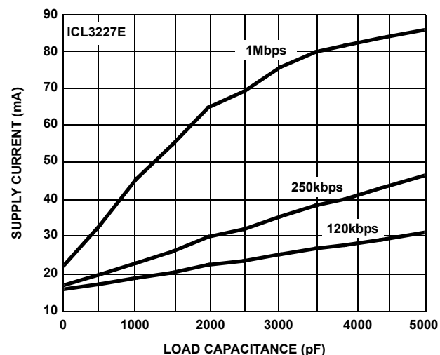
FIGURE 21. SUPPLY CURRENT vs LOAD CAPACITANCE WHEN TRANSMITTING DATA
