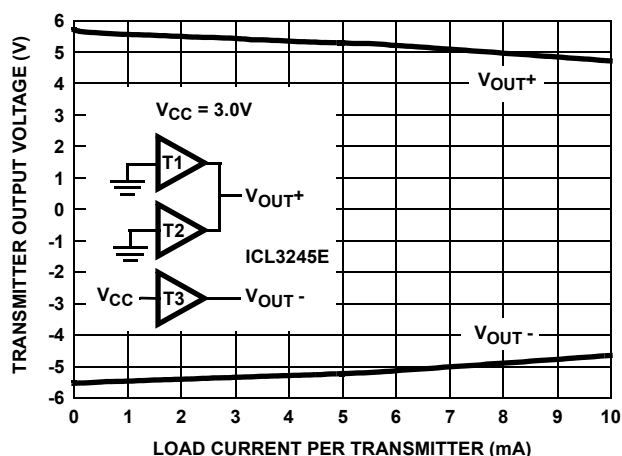
FIGURE 14. TRANSMITTER OUTPUT VOLTAGE vs LOAD CURRENT (PER TRANSMITTER, i.e., DOUBLE CURRENT AXIS FOR TOTAL V_{OUT+} CURRENT)
