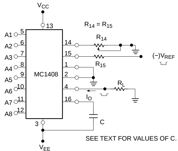
Figure 4. Negative V_{REF}
