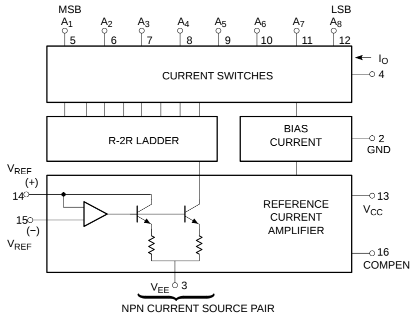
Figure 1. Block Diagram
