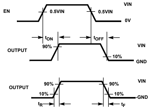
FIGURE 27. TRANSIENT WAVEFORM MEASUREMENT POINTS
