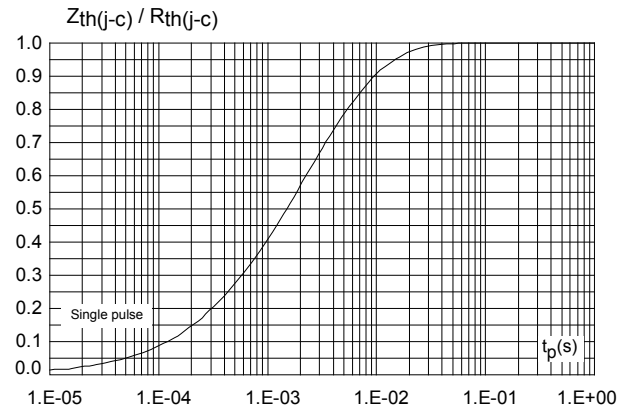
Figure 6. Relative variation of thermal impedance junction to case versus pulse duration (TO-220AC, DPAK HV 2L, D 2 PAK)
