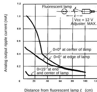
Retroreflective Type E3SA-RS50C43A
