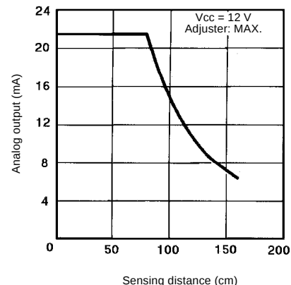
Polarized Retroreflective Type E3SA-RS50C43A
