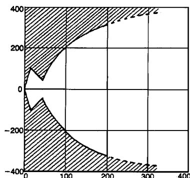
Through-Beam Type E3SA-2C43A Without Slit
