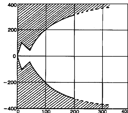
Through-Beam Type E3SA-2C43A With Slit
