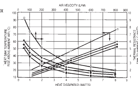
669-52AB 12 x 12 PIN MATRIX
