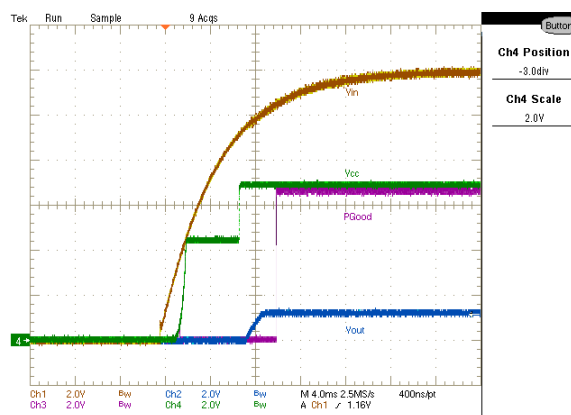
Figure 39: Startup with full load, VCC signal CH1:Vin, CH2:Vout, CH3:PGood, CH4:VCC
