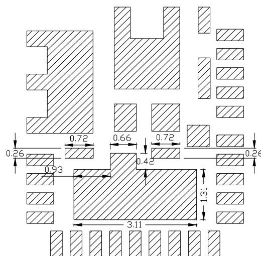
PCB PAD SPACING (DETAIL 2)
