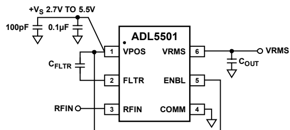
Figure 40. Basic Connections for ADL5501
