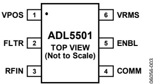
Figure 3. Pin Configuration
