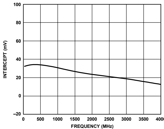
Figure 39. Intercept vs. Frequency, Supply 5 V
