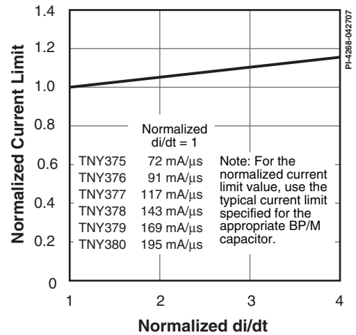
Figure 24. Current Limit vs. di/dt.
