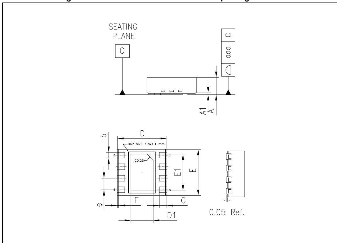
Figure 28. DFN8 2x2 mm wettable flanks package outline
