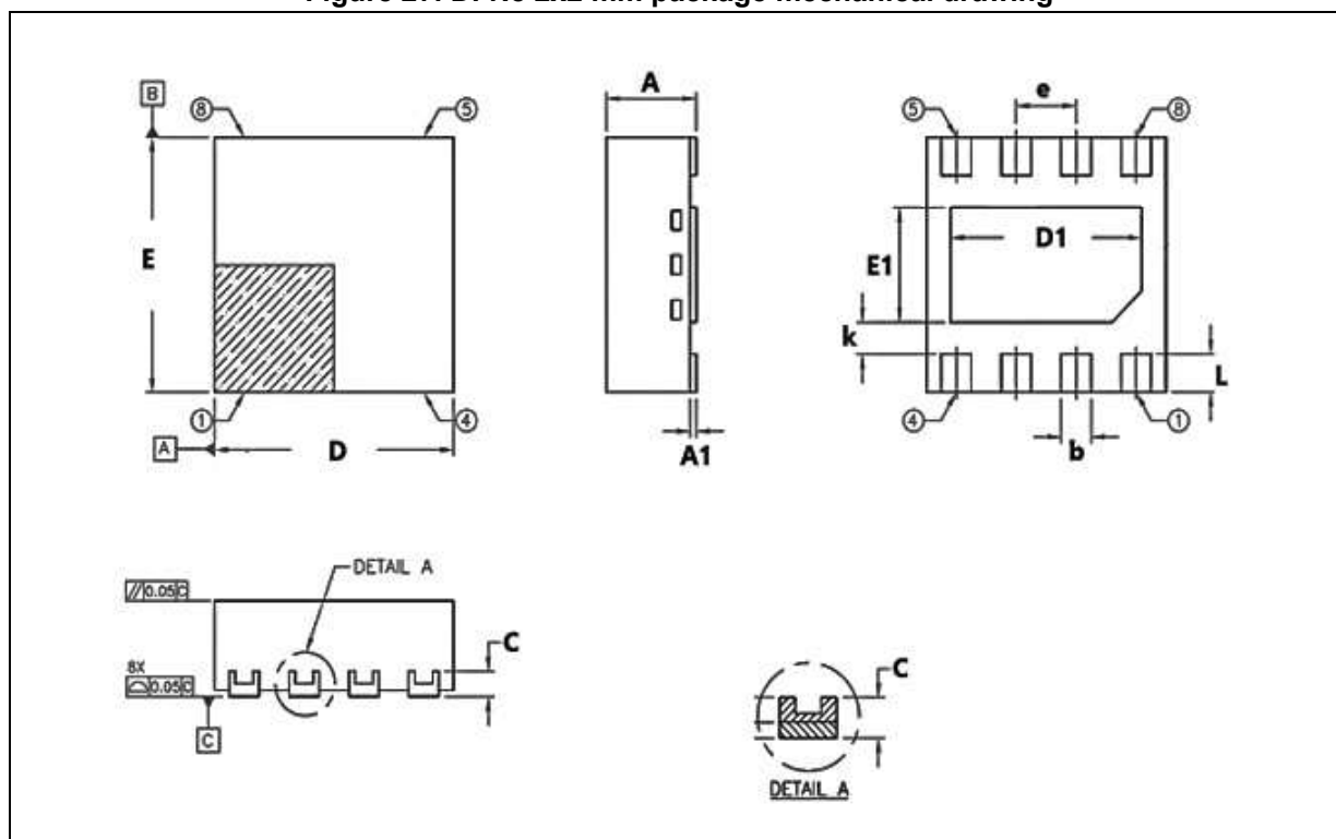
Figure 27. DFN8 2x2 mm package mechanical drawing
