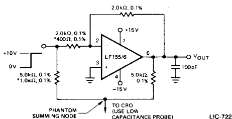
Settling Time Test Circuit
