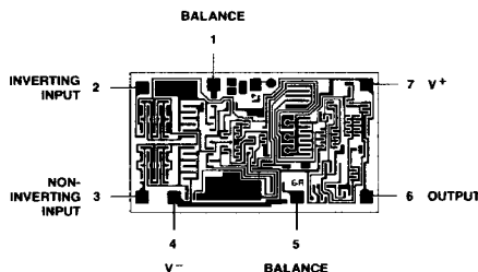
Metallization and Pad Layout
