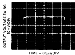
LF156 Small Signal Pulse Response, A_V = +1
