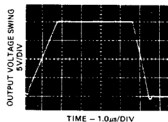
LF156 Large Signal Pulse Response, A_V = +1
