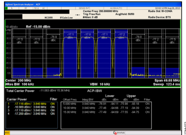
Figure 18. 4-Carrier WCDMA ACLR Performance, f_{IF} = 200 MHz, f_{DAC} = 1228.8 MHz
