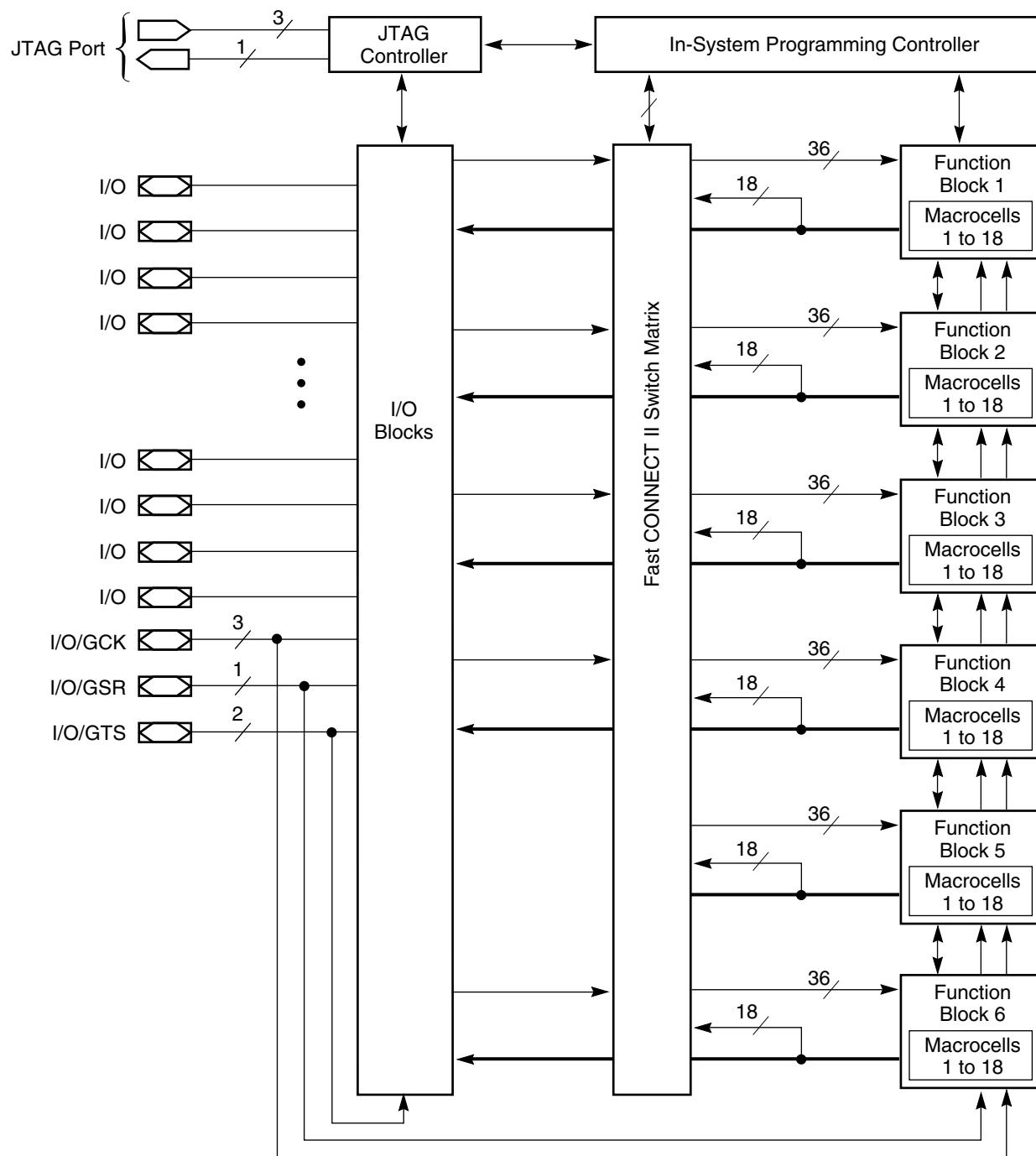
Figure 2: XC95108 Architecture
