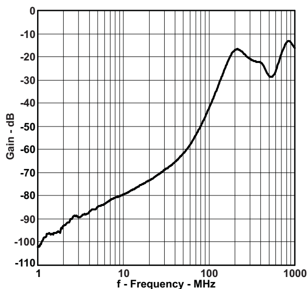
Figure 14. Crosstalk Adjacent vs Frequency ( V_+ = 1.8 V)
