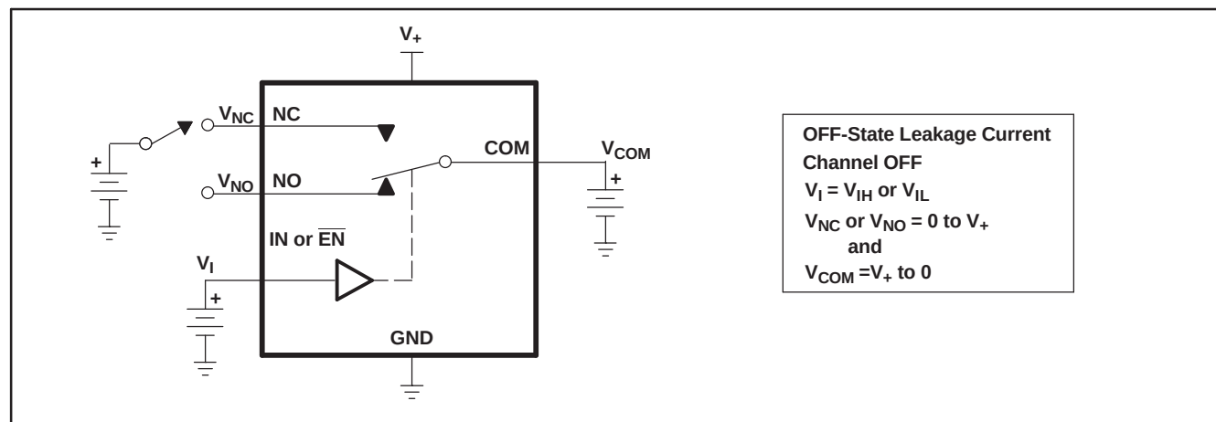
Figure 20. OFF-State Leakage Current ( I_{COM(OFF)} , I_{NC(OFF)} , I_{NO(OFF)} )
