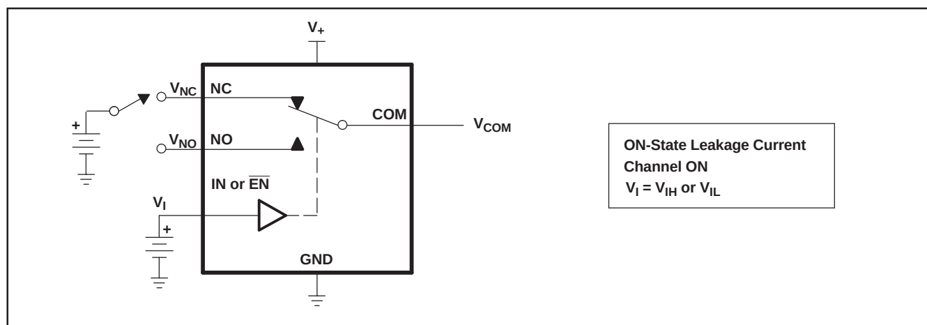
Figure 21. ON-State Leakage Current ( I_{COM(ON)} , I_{NC(ON)} )
