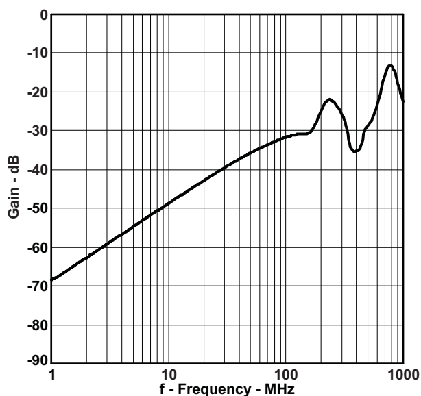
Figure 13. OFF Isolation vs Frequency ( V_+ = 1.8 V)
