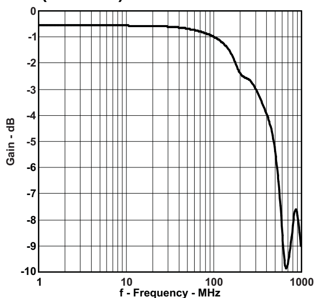
Figure 12. Gain vs Frequency Bandwidth ( V_+ = 1.8 V)
