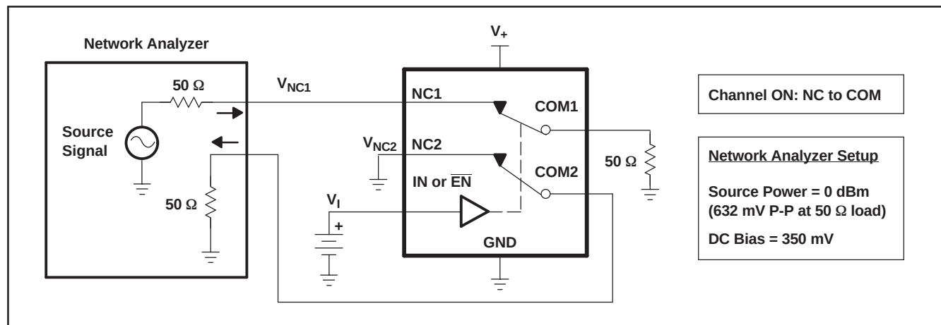
Figure 27. Crosstalk Adjacent
