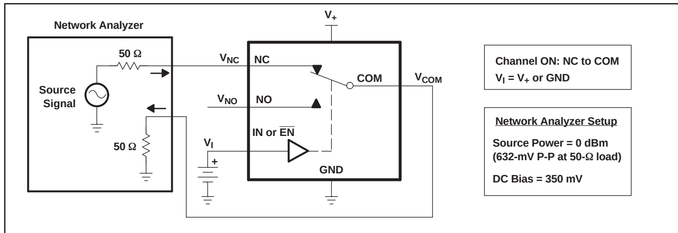
Figure 24. Bandwidth (BW)
