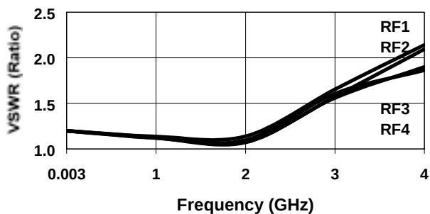
RFC On VSWR @ 25 °C
