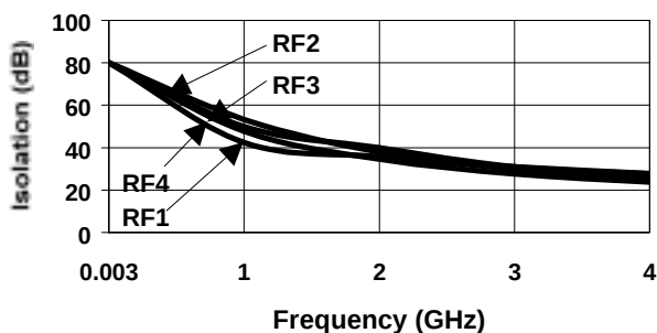
Isolation (dB) @ 25 °C
