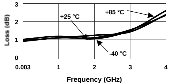
Loss Variation Over Temp. (dB)
