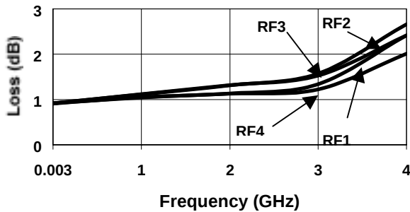
Insertion Loss (dB) @ 25 °C
