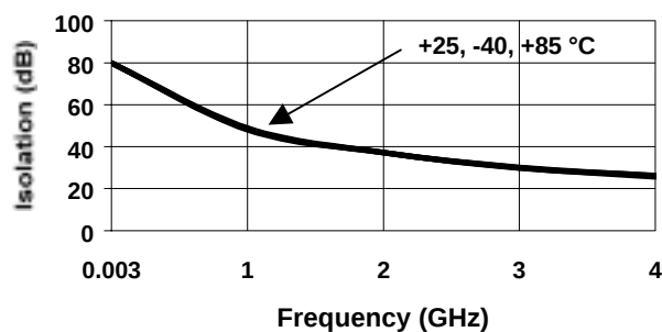
Isolation Temperature Variation (dB)
