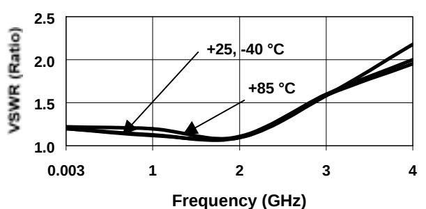
RFC On VSWR Temperature Variation
