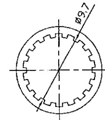
LOCK WASHER
