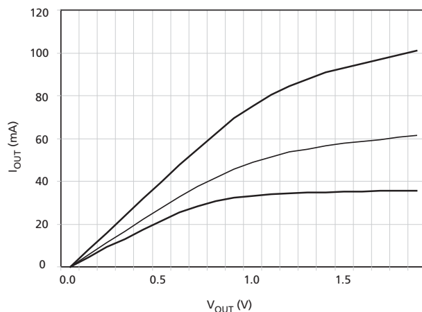
Figure 15: Full Strength Pull-Down Characteristics
