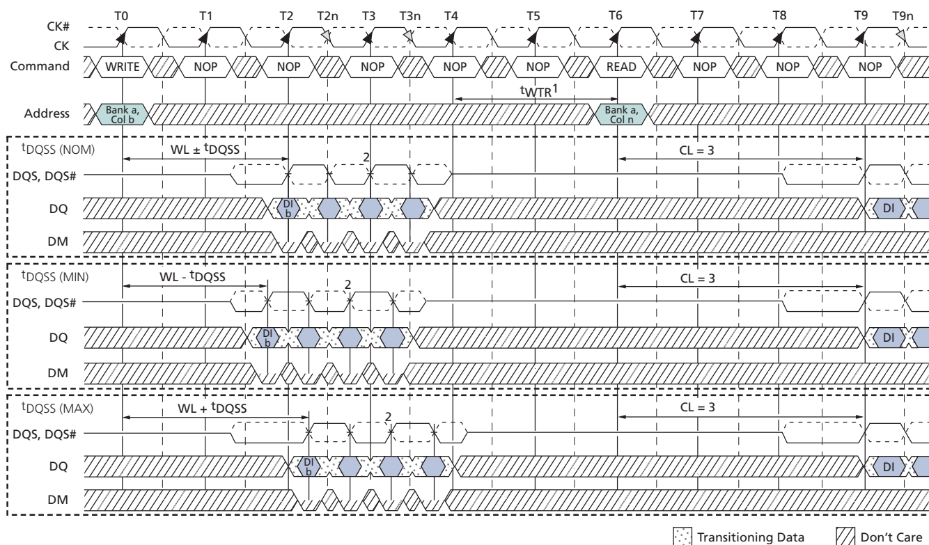
Figure 60: WRITE-to-READ
