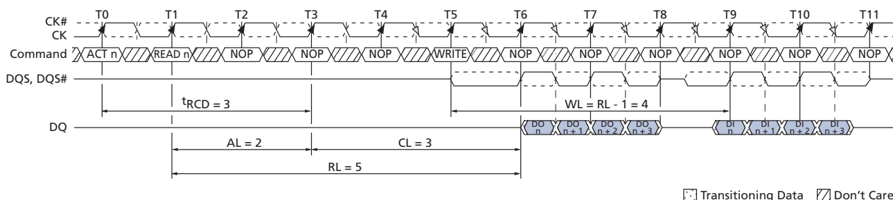
Figure 48: READ-to-WRITE
