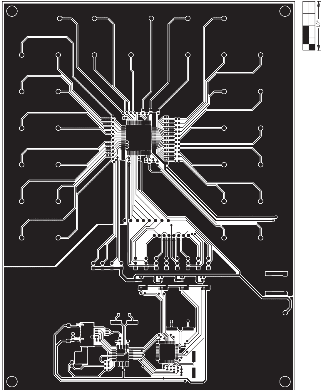
Figure 5. MAX9675 EV Kit PCB Layout—Component Side
