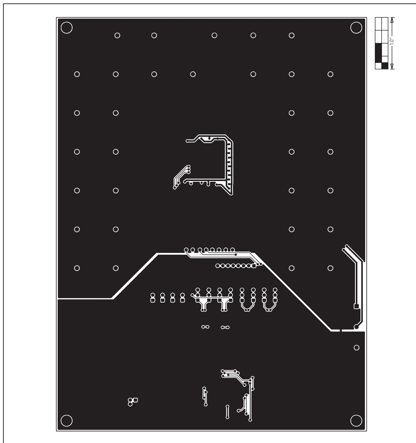
Figure 6. MAX9675 EV Kit PCB Layout—Solder Side
