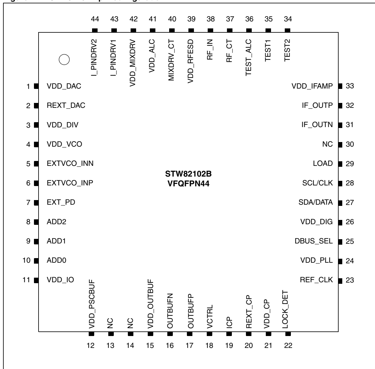
Figure 2. STW82102B pin configuration
