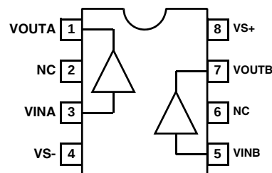
EL5221 (8 LD MSOP) TOP VIEW
