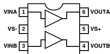
EL5221 (6 LD SOT-23) TOP VIEW
