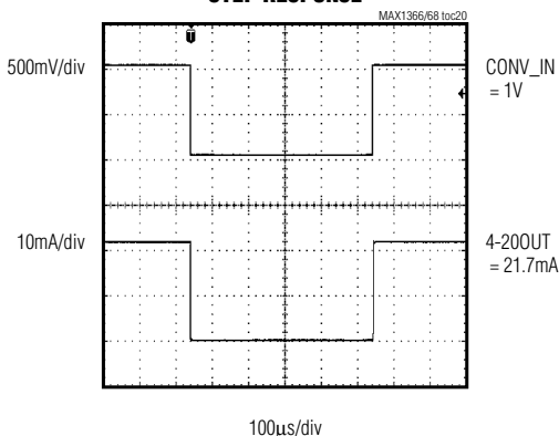
STEP RESPONSE
