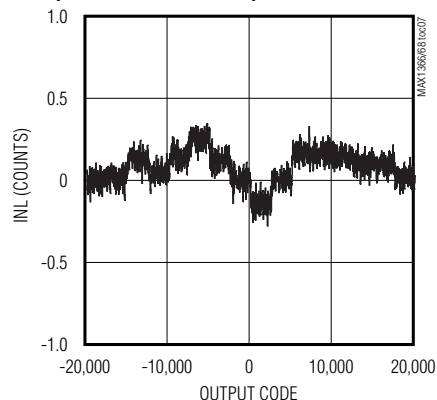
MAX1366 (±200mV INPUT RANGE) INL vs. OUTPUT CODE
