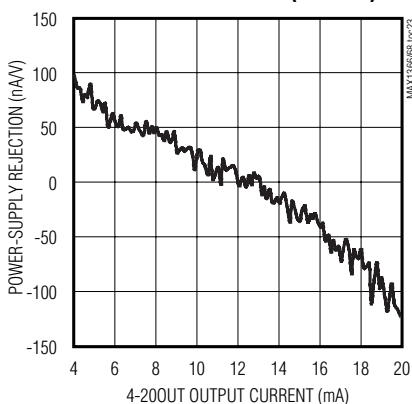
POWER-SUPPLY REJECTION vs. CURRENT OUTPUT (4-200UT)
