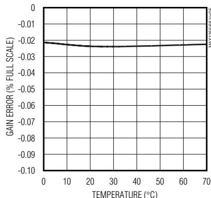
MAX1366 GAIN ERROR vs. TEMPERATURE
