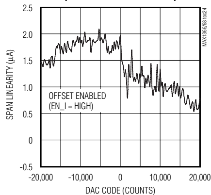
4-200UT vs. DAC CODE (4-200UT SPAN LINEARITY)
