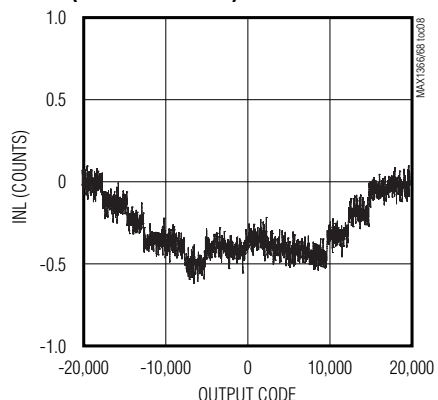
MAX1366 (±2V INPUT RANGE) INL vs. OUTPUT CODE
