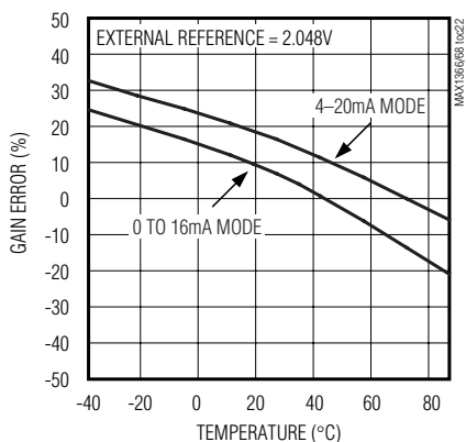
4-200UT GAIN ERROR vs. TEMPERATURE
