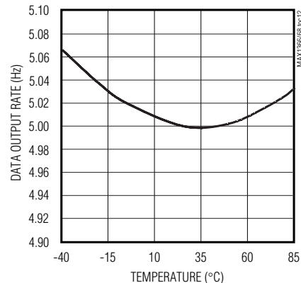
DATA OUTPUT RATE vs. TEMPERATURE
