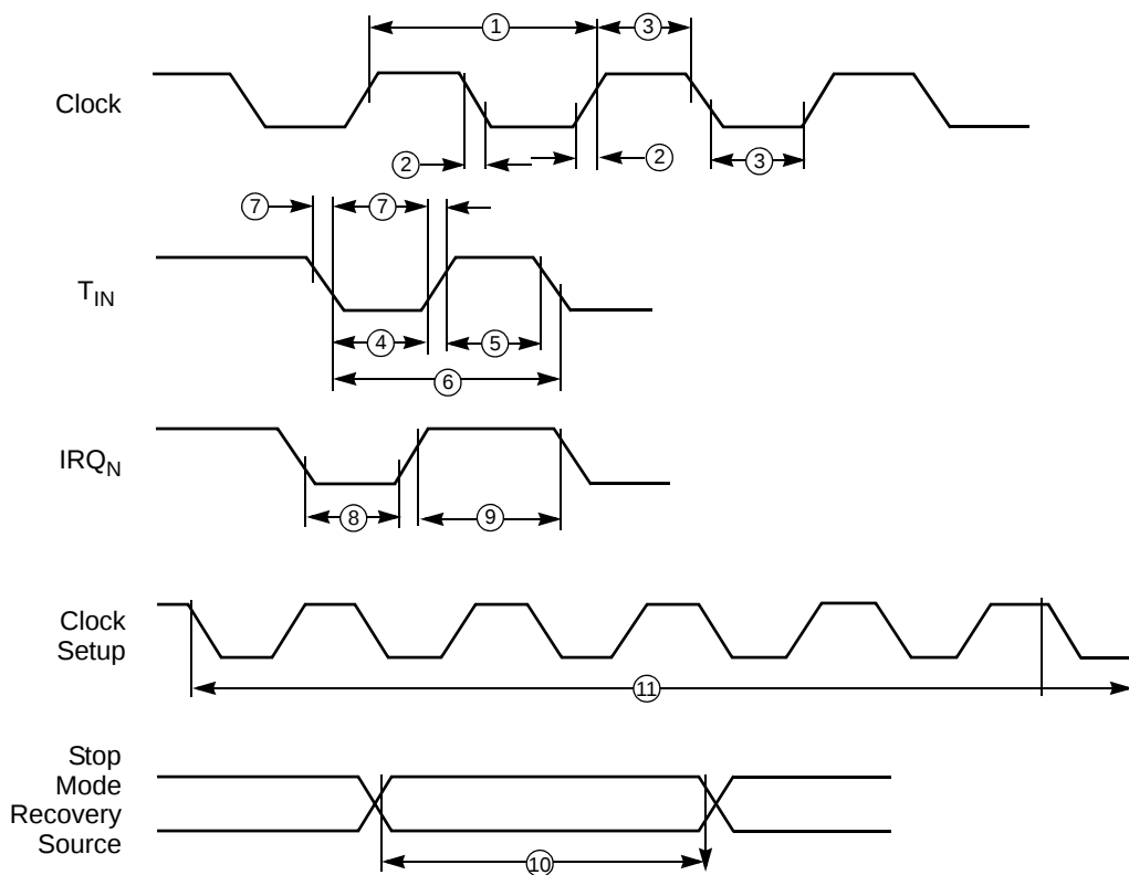
Figure 5. Timing Diagram
