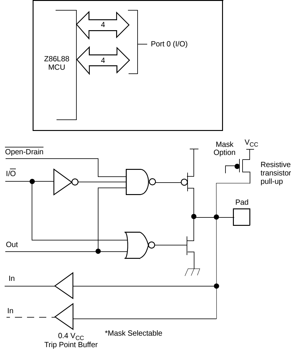
Figure 6. Port 0 Configuration
