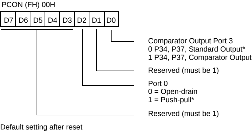
Figure 19. Port Configuration Register (PCON)—(0F) 0H: Write Only
