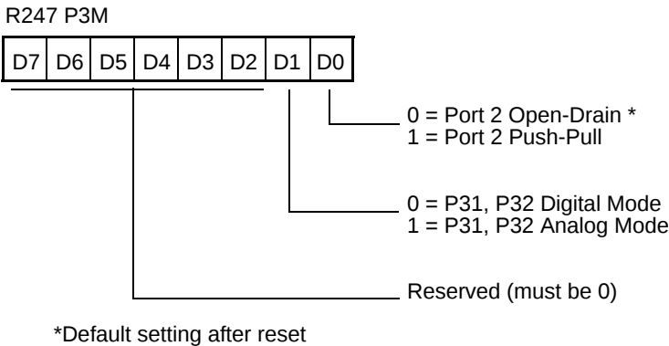
Figure 21. Port 3 Mode Register—F7H: Write Only
