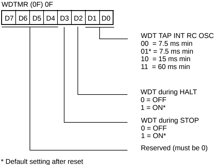
Figure 18. Watch-Dog Timer Register—(0F) 0FH: Write Only
