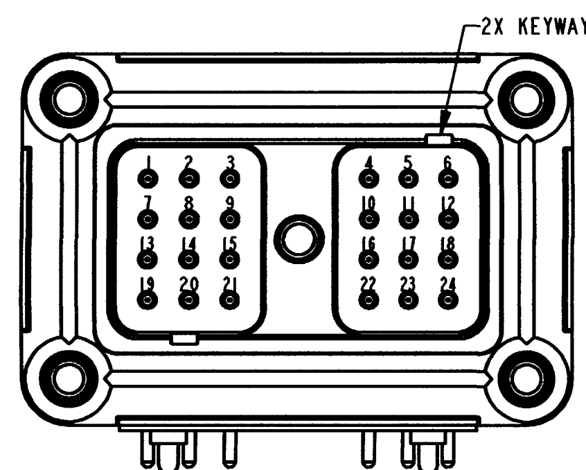
ARRANGEMENT -B- DRC13-24PB
