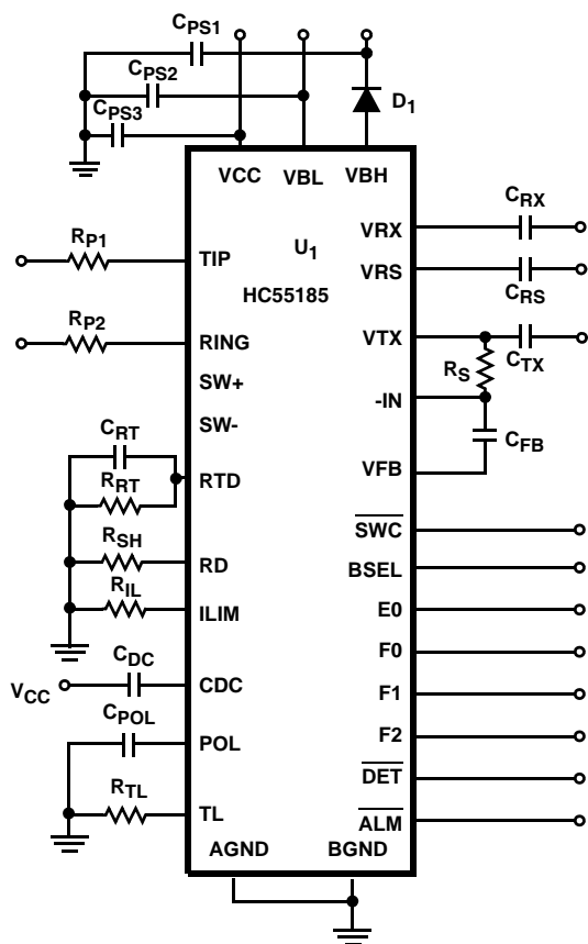
FIGURE 15. HC55185 BASIC APPLICATION CIRCUIT
