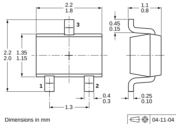
Fig 15. Package outline PDTA143XU (SOT323/SC-70)
