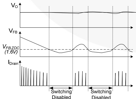
Figure 31. Burst-Mode Operation
