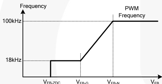
Figure 30. PWM Frequency
