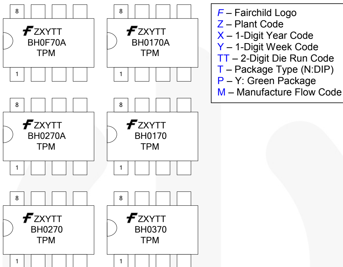
Figure 4. Pin Configuration and Top Mark Information
