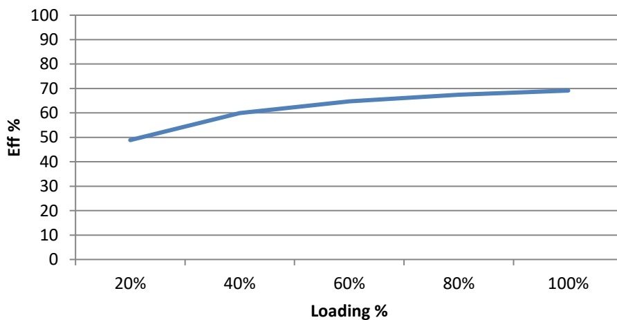
AM1DR-2405SZ Efficiency vs. Loading
