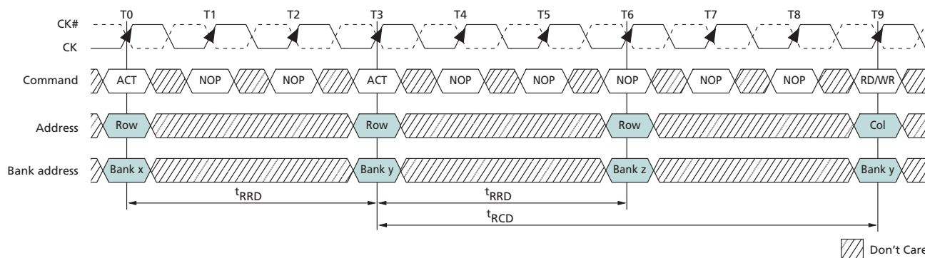
Figure 44: Example: Meeting t_{\text{RRD}} (MIN) and t_{\text{RCD}} (MIN)
