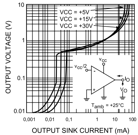
Figure 10. Output characteristics (sink)
