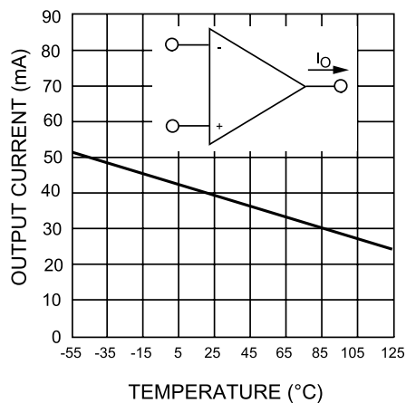
Figure 5. Current limiting
