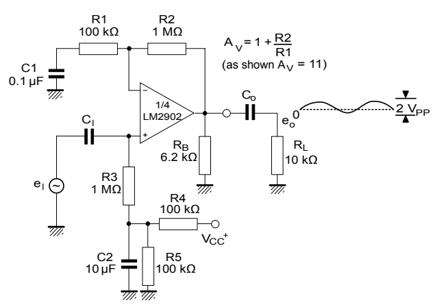
Figure 24. AC coupled non-inverting amplifier
