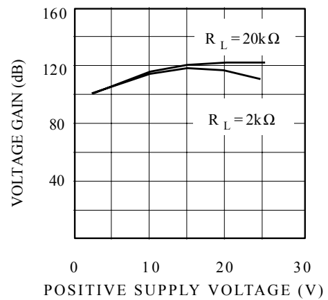
Figure 16. Voltage gain
