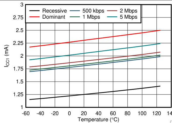
Figure 6. I_{CC1} vs Datarate
