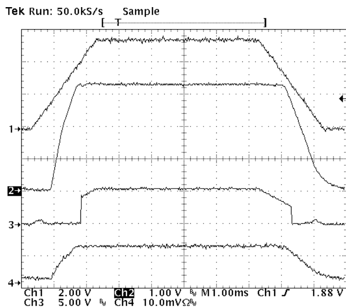
Figure 3–1. Input Voltage Ramp
