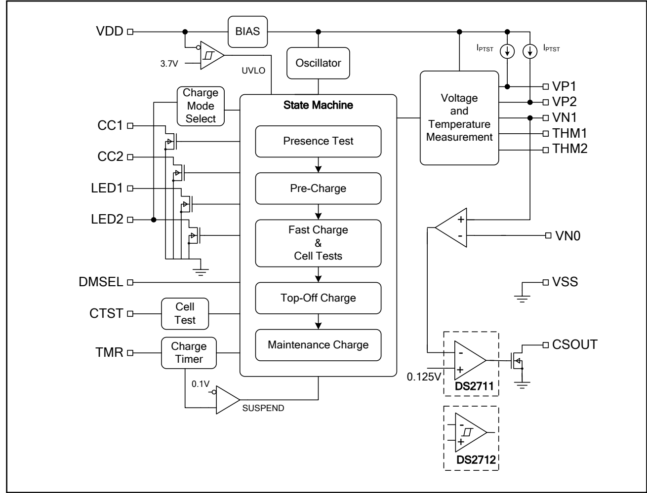
Figure 1. Block Diagram
