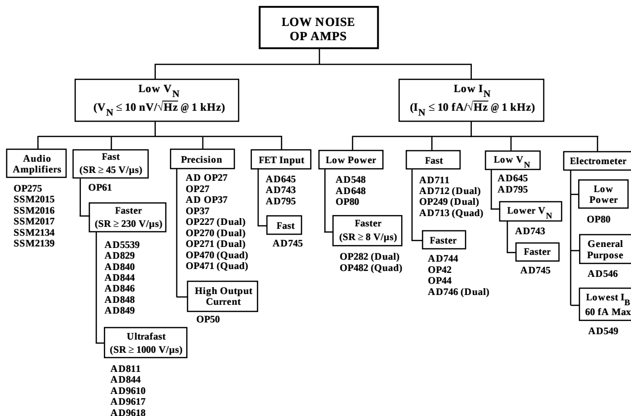
Low Noise Op Amp Selection Tree
