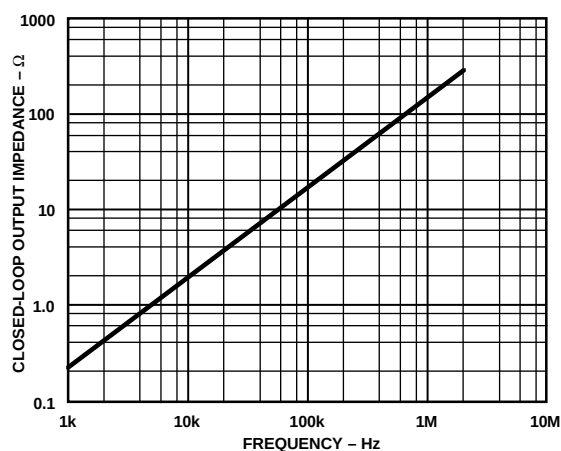
Figure 20. Closed-Loop Output Impedance vs. Frequency
