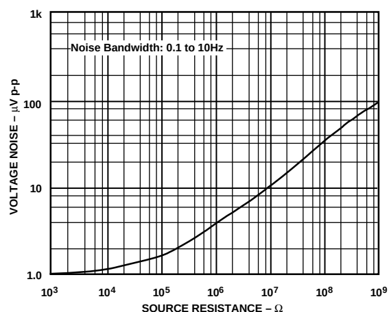
Figure 10. Input Voltage Noise vs. Source Resistance
