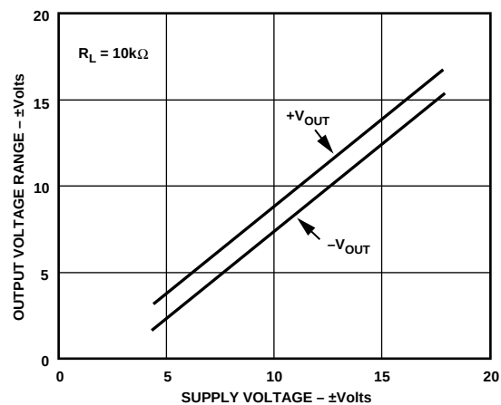
Figure 2. Output Voltage Range vs. Supply Voltage
