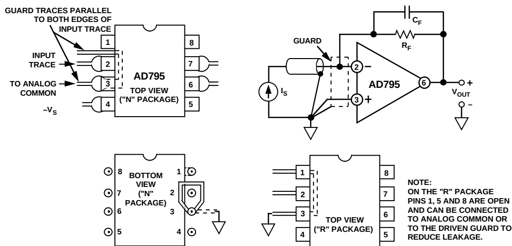
Figure 31. Guarding Scheme-Inverter
