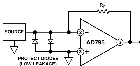
Figure 42. Input Voltage Clamp with Diodes
