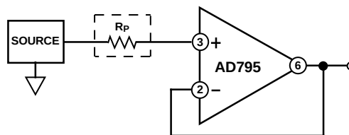
Figure 41. Follower with Input Current Limit
