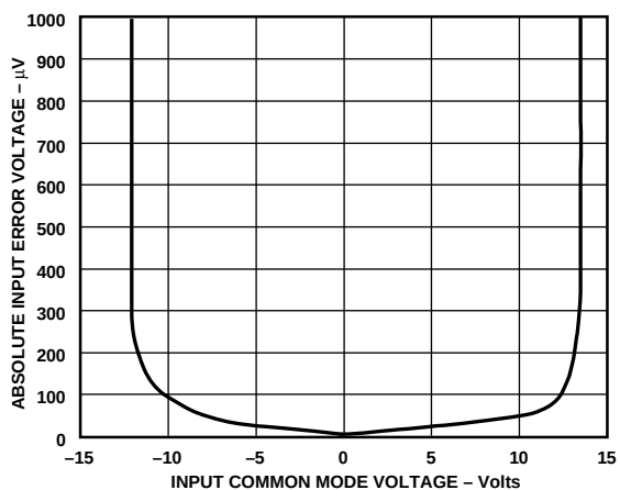
Figure 15. Absolute Input Error Voltage vs. Input Common-Mode Voltage
