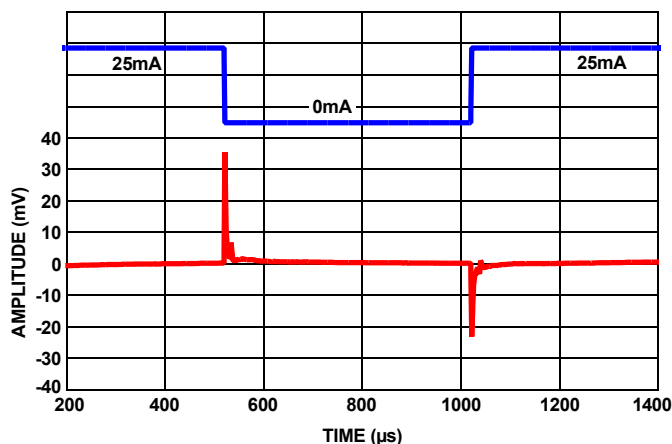
FIGURE 61. LOAD TRANSIENT RESPONSE AT 25mA LOAD AT 1μF
