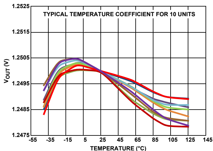
FIGURE 34. V_{OUT} vs TEMPERATURE
