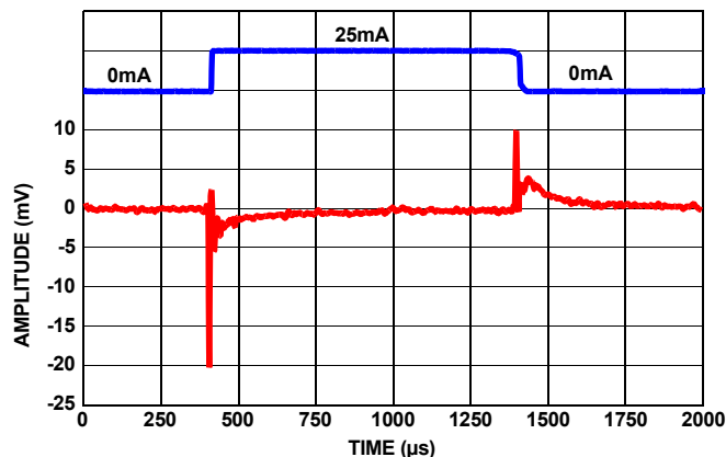
FIGURE 27. LOAD TRANSIENT RESPONSE AT 25mA LOAD AT 1μF
