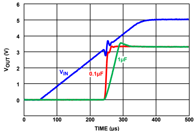
FIGURE 114. TURN-ON TIME
