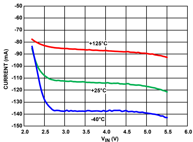
FIGURE 18. SHORT CIRCUIT TO GND
