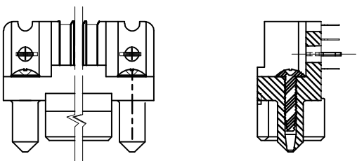
SECTION U-U
