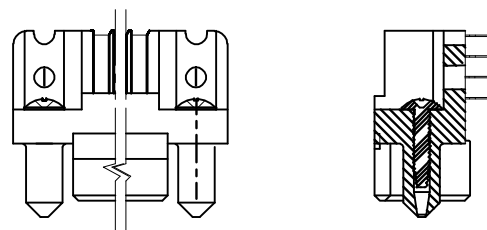
SECTION U-U
